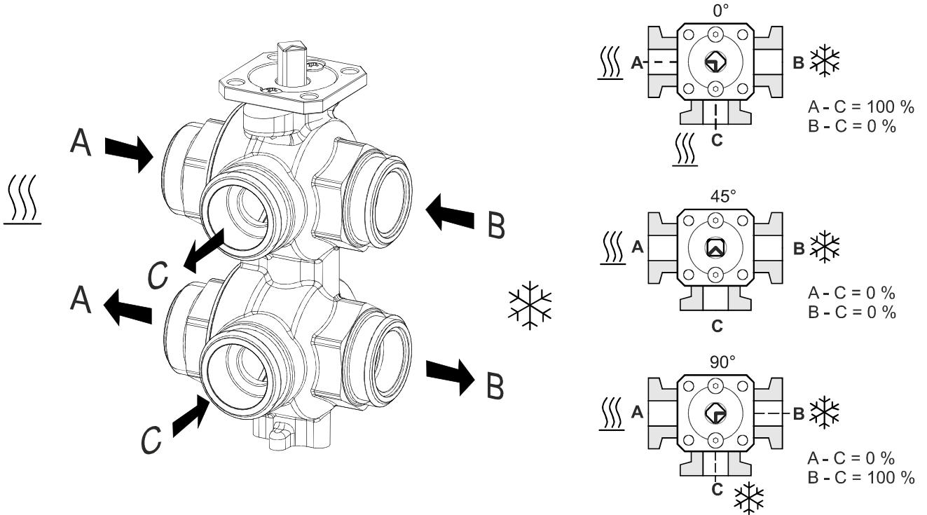
Example: VWG41.20-1.6-2.5
