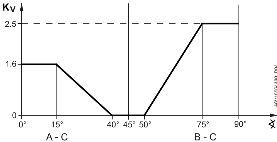
Example: VWG41.20-1.6-2.5
