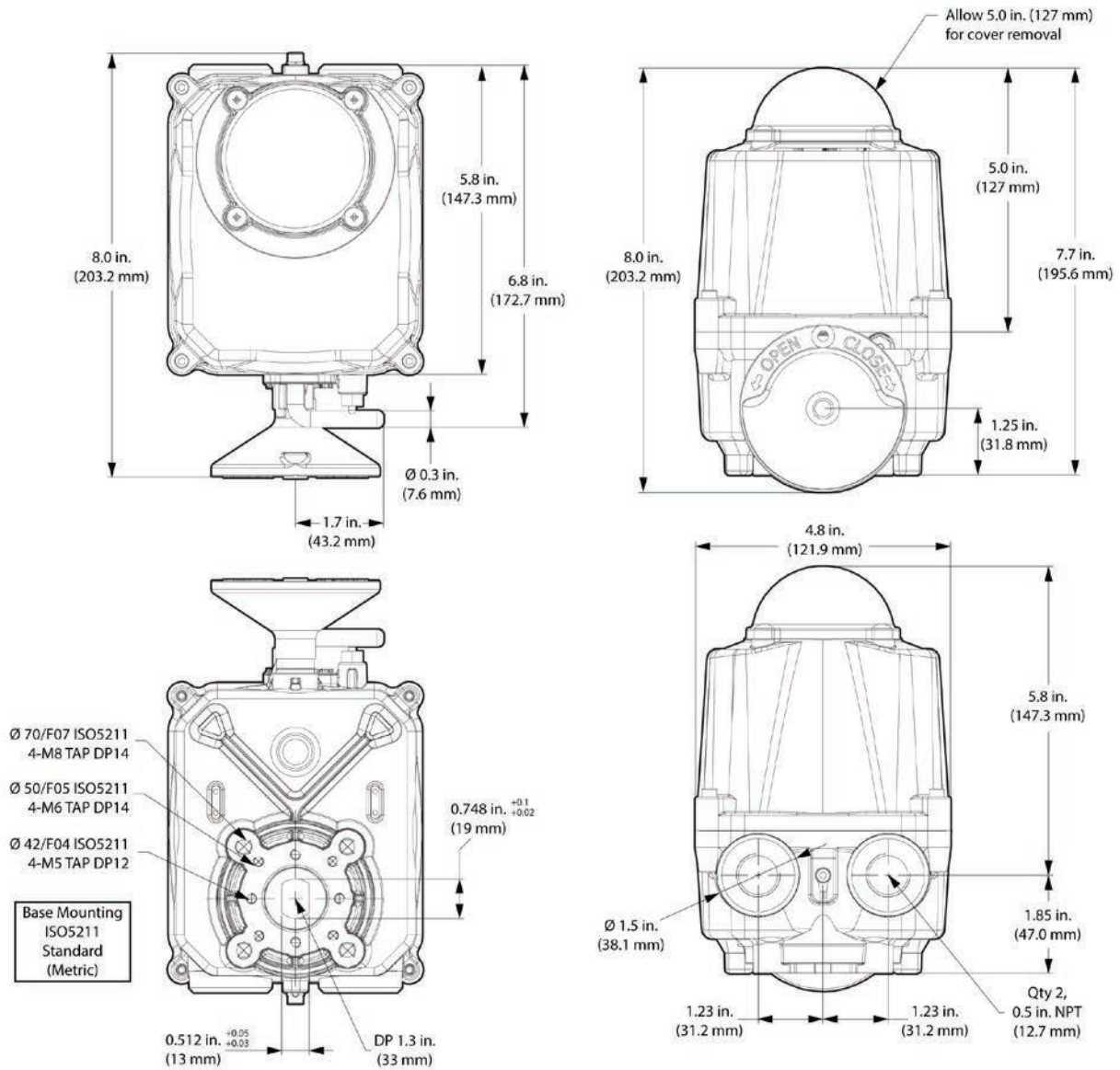
Figure 5. Model Axx6.530 Dimensions in Inches (Millimeters).
