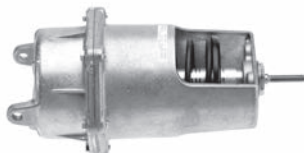
331-3060 No. 6 Pneumatic Actuator, pivot mounting type
