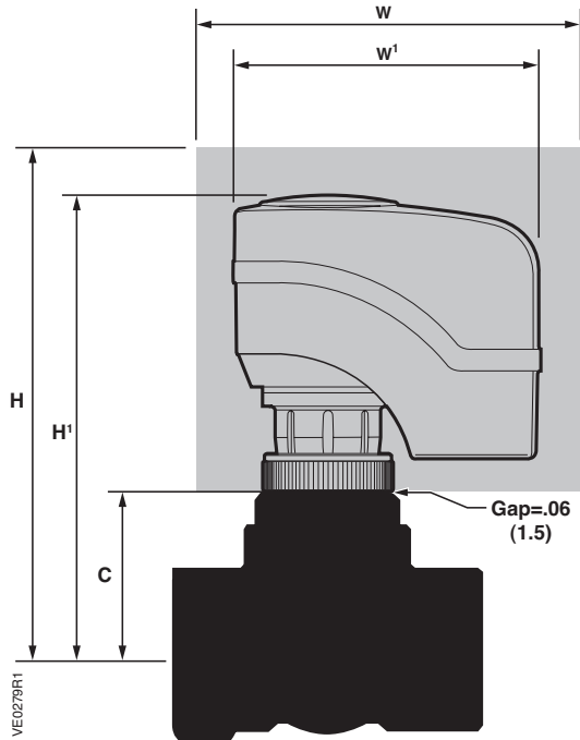
SSA81U Series Actuator: Service Envelope for 2-Way Valve Assembly
